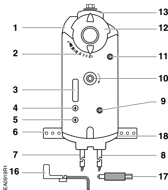
Figure 1. Components of the GMA Spring Return Actuator.
