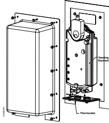
Figure 7. Heater/Weather Shield Assembly.
